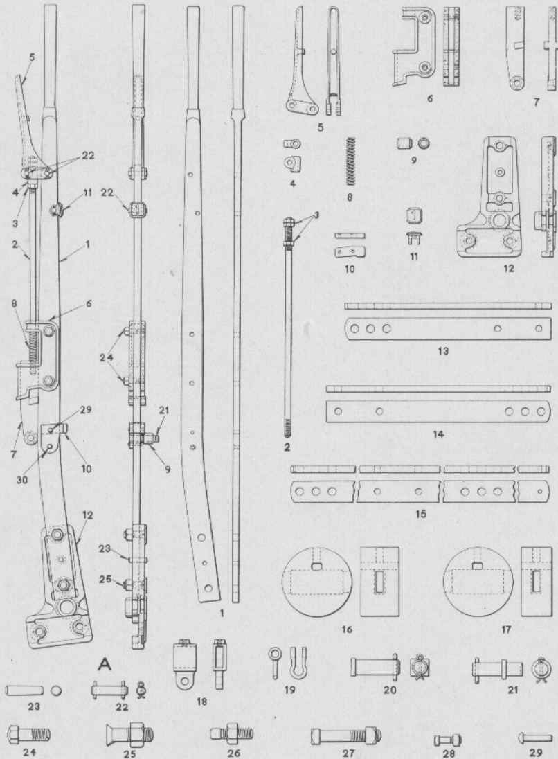
LEVERS AND DETAILS FOR STYLE "A" INTERLOCKING MACHINE
